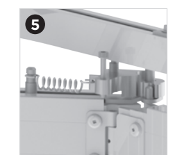
Ensemble de cames de compression
